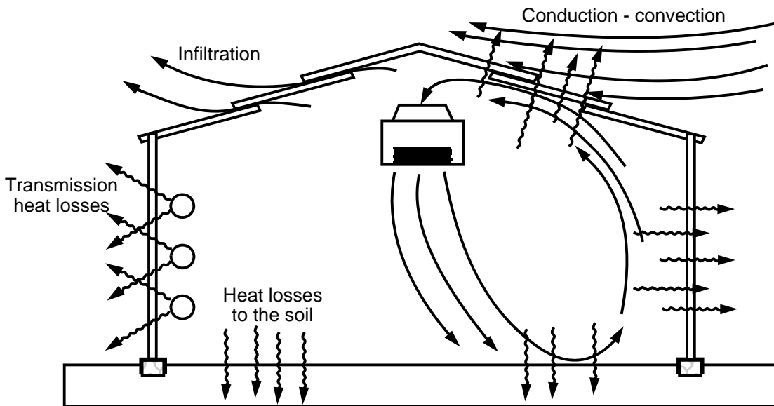
HEAT LOSSES
