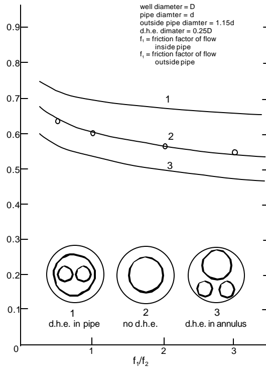
Figure 8. Optimum diameter of the convection promoting pipe for varying friction factor ratio; in the three cross-sections, f_2/f_1 = 2 . Refer to text for derivation of the 4 points and the curves.
