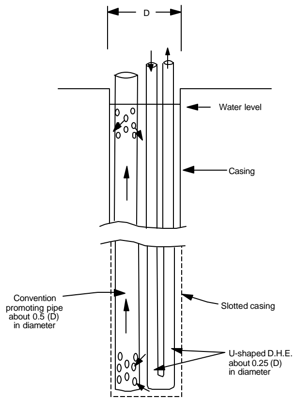
Figure 6. Convector promotion and DHE (New Zealand type).
