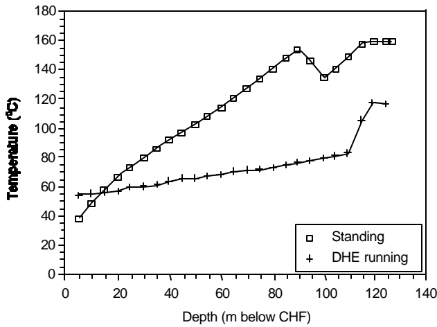
Figure 11. Downhole temperature.
