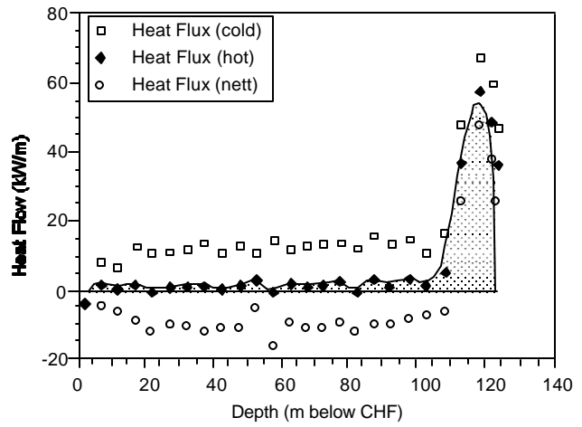
Figure 12. Heat flux (1.2 l/s).
