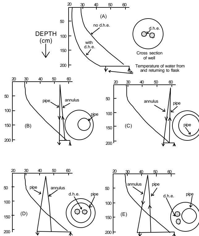
Figure 9. Characteristic temperature and flow regimes observed in a laboratory model of a well; configuration of convection promoting pipe and/or DHE is shown in the cross-section in each case.
