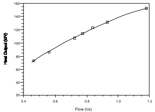
Figure 13. Heat output vs. flow rate.
