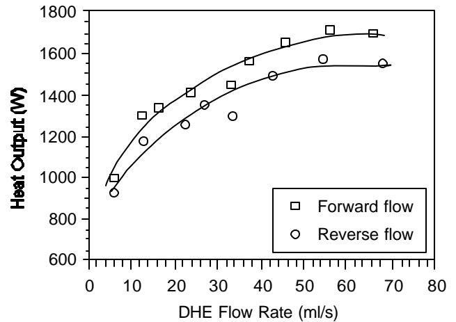
Figure 17. Heat output vs. DHE flow (32-mm promoter)(Cross-flow rate 31.4 ml/s).
